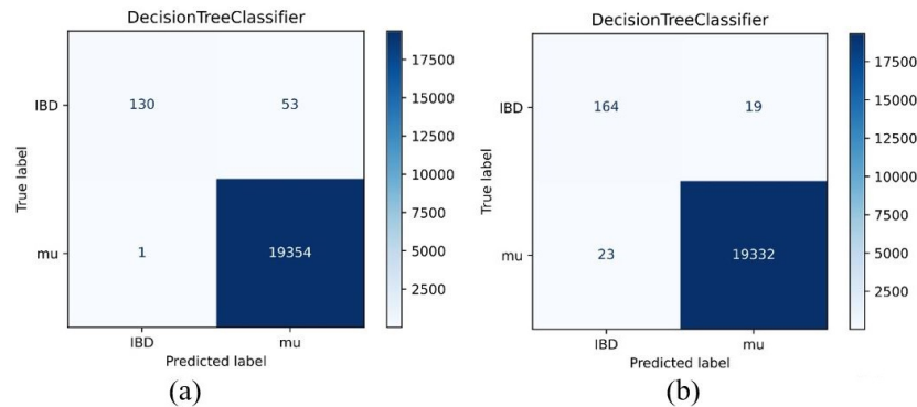
Figure 12: Confusion matrix (a) before and (b) after the over-sampling.
