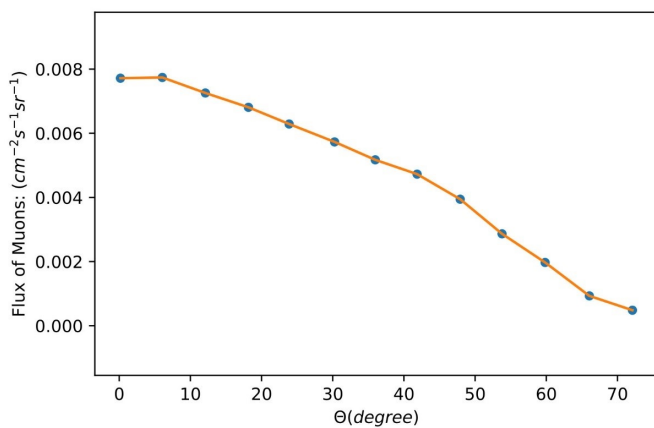
Figure 6: Angular distribution of cosmic muons near Bushehr (Arneodo et al., 2019).
