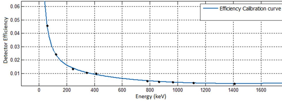
Figure 2: HPGe efficiency calibration curve.
