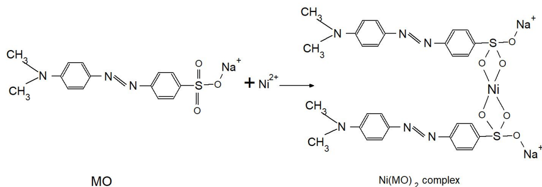
Figure 1: Chemical structure of Ni(MO) 2 complex.
