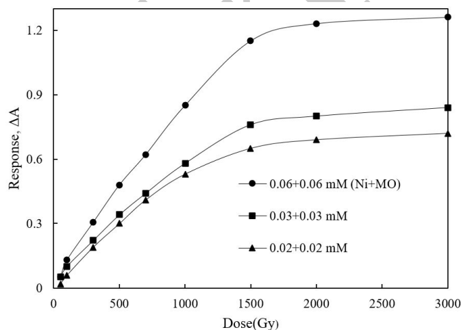
Figure 5: The dose-response curves of the Ni/ MO complex solution at 460 nm for different concentrations: \Delta A = A_0 - A_i where A_0 and A_i are the optical absorptions at 460 nm wavelength for the unirradiated and irradiated solution, respectively.
