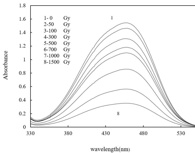
Figure 4: The absorption spectra of Ni/ MO complex solution irradiated to different absorbed doses, [0.06 + 0.06 mM].
