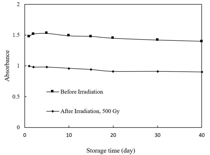
Figure 6: Stability of the liquid Ni/MO complex before and after irradiation as a function of storage time (stored in environmental conditions for 0.06 + 0.06 mM [Ni+MO] concentration).
