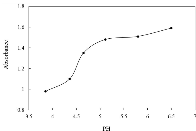
Figure 2: Effect of pH on the absorbance of the Ni/MO solution at 0.06 + 0.06 mM concentration [Ni+MO].
